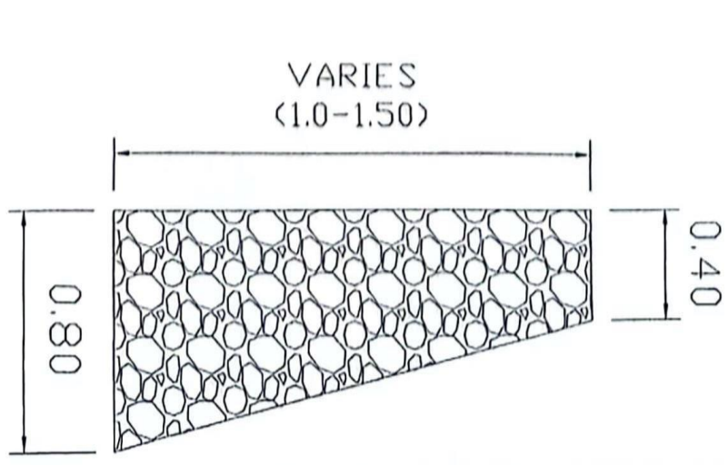
STONE MASONRY AR SECTION SCALE NTS
