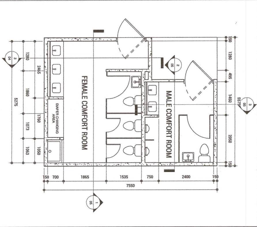
1 GROUND FLOOR PLAN 1 : 50
