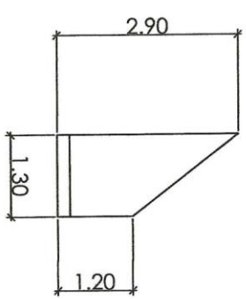
SECTION - WINGWALL SCALE NTS
